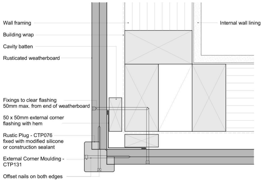
Rusticated – External 90° Corner – Moulding
