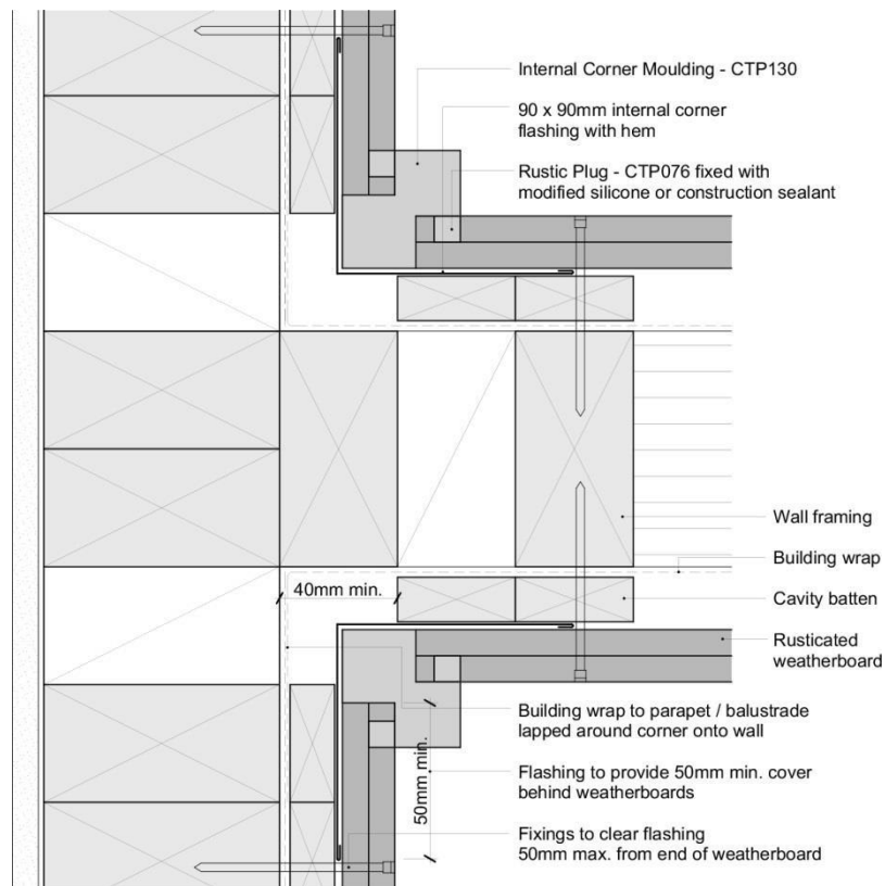
Rusticated – Parapet Balustrade Intersection With Wall – Moulding
