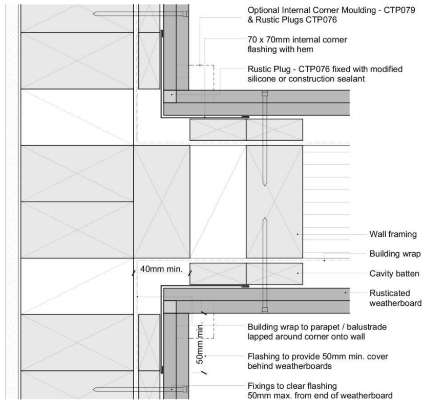
Rusticated – Parapet Balustrade Intersection With Wall – Butted
