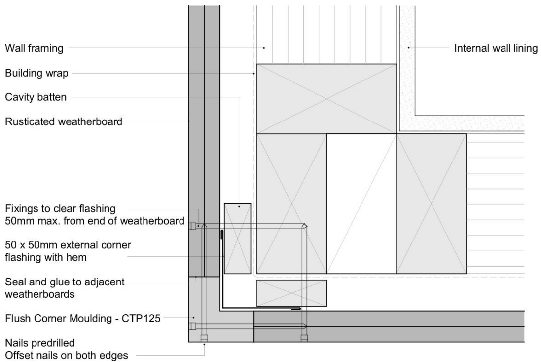
Rusticated – External 90° Corner – Flush Moulding
