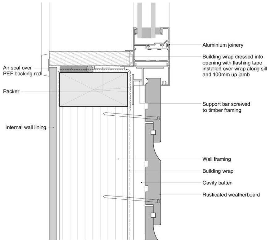
Rusticated – Window Sill
