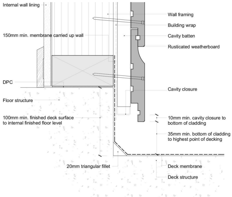
Rusticated – Enclosed Deck – Concrete Substrate
