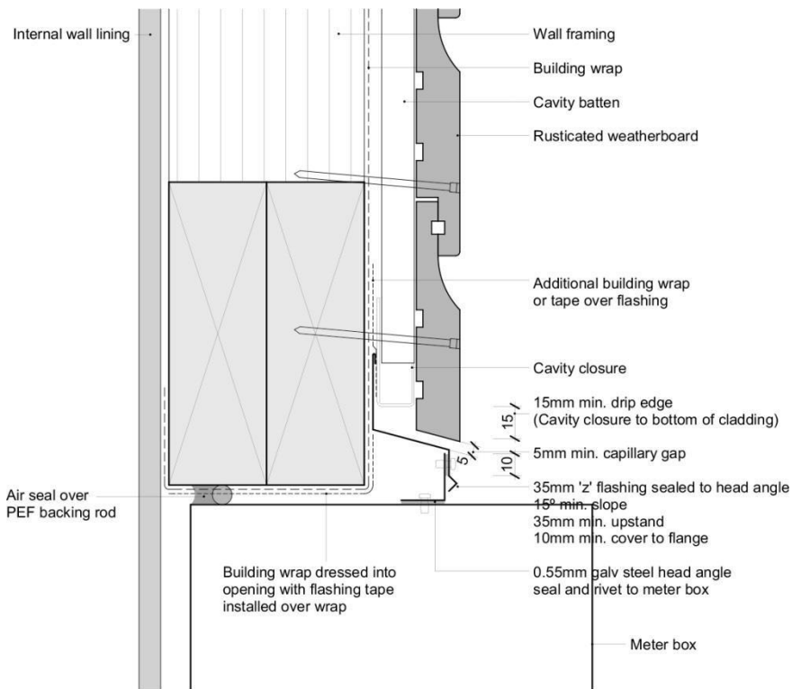
Rusticated – Meter Box Head
