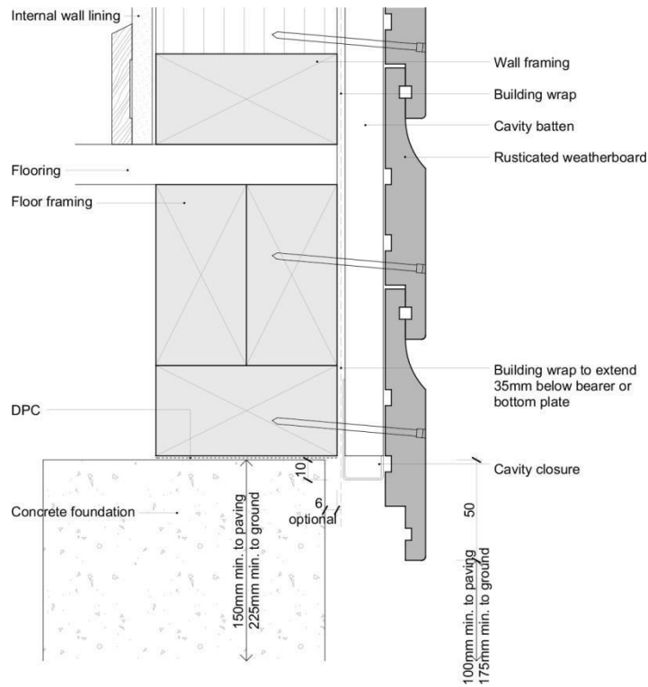
Rusticated – Base Of Wall – Timber Floor
