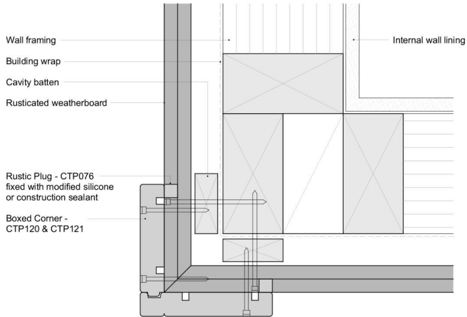
Rusticated – External 90° Corner – Boxed
