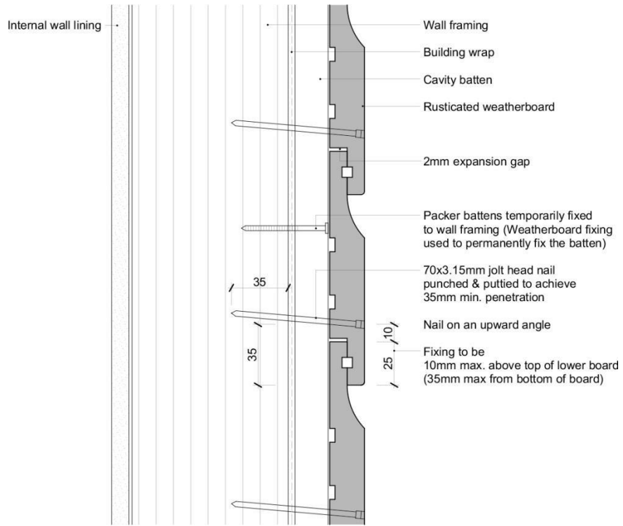
Rusticated – Packer Cavity Batten
