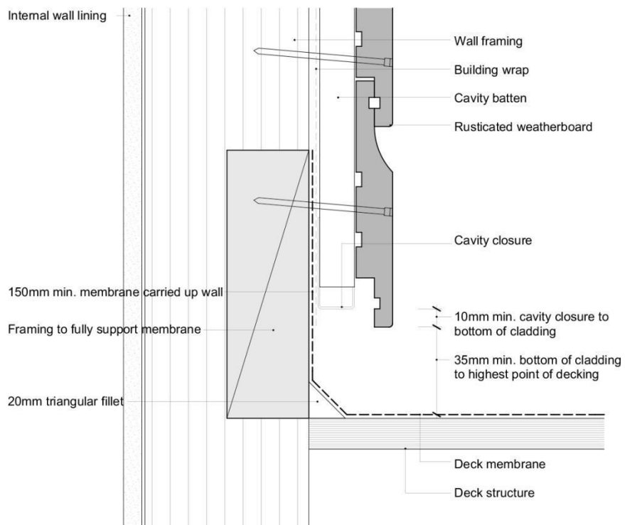
Rusticated – Enclosed Deck – Timber Substrate
