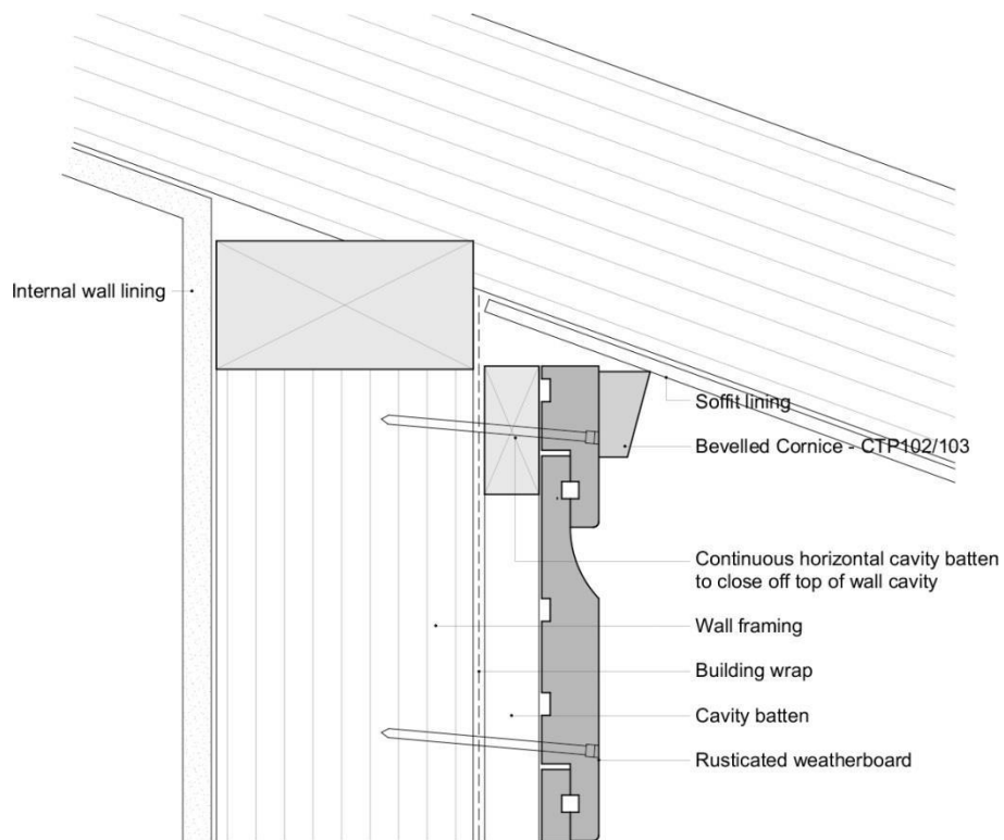
Rusticated – Top Of Wall – Sloping Soffit
