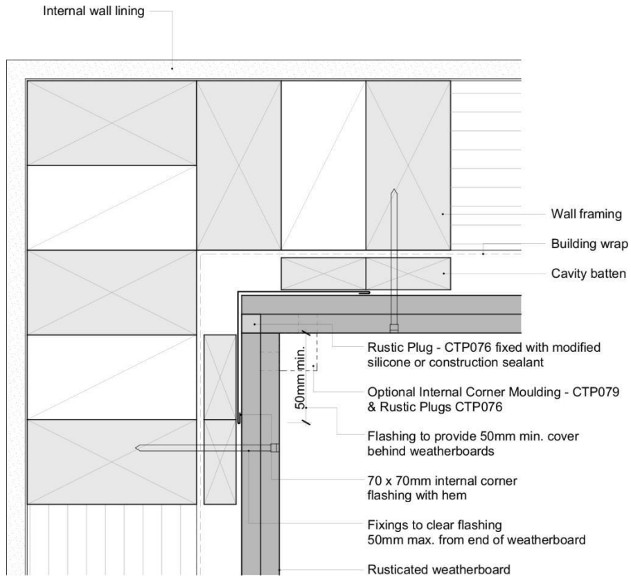
Rusticated – Internal 90° Corner – Butted
