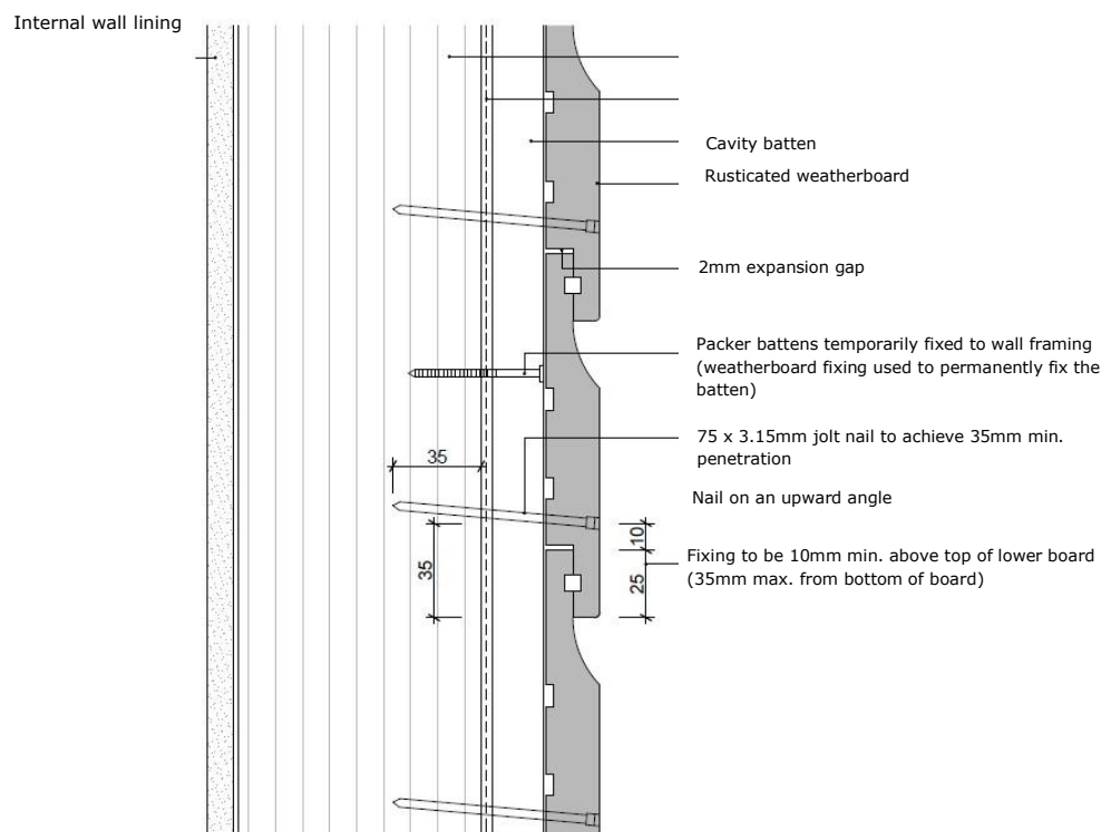
Rusticated Fixing
