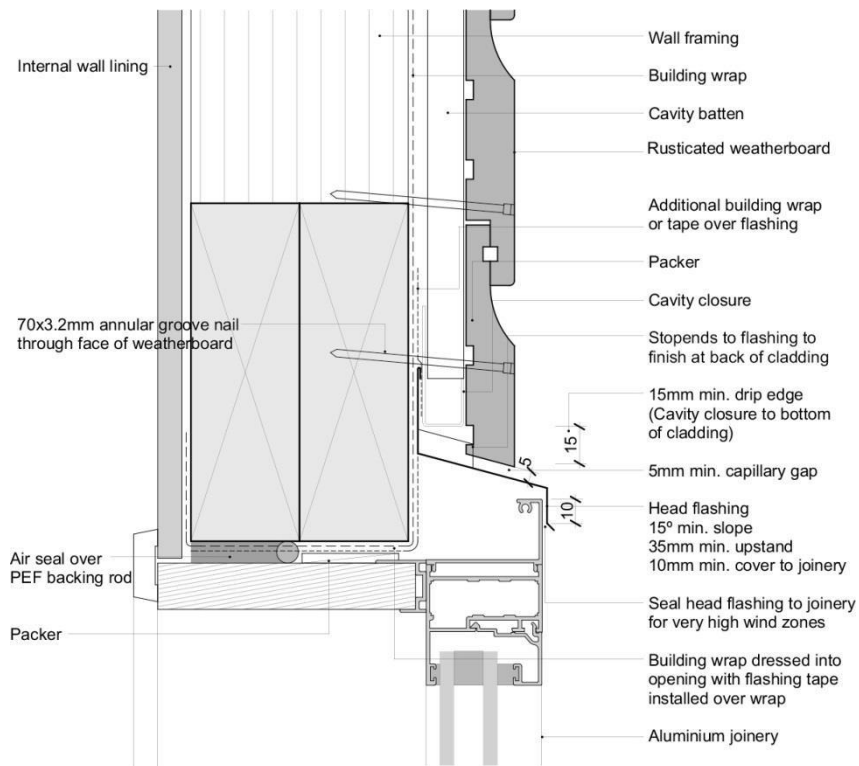
Rusticated – Window Head
