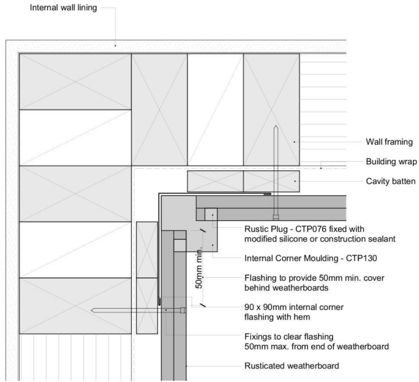
Rusticated – Internal 90° Corner – Moulding
