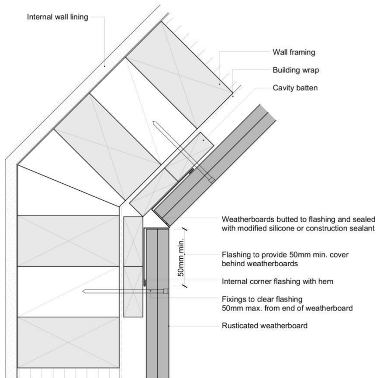
Rusticated – Internal 135° Corner – Flashing
