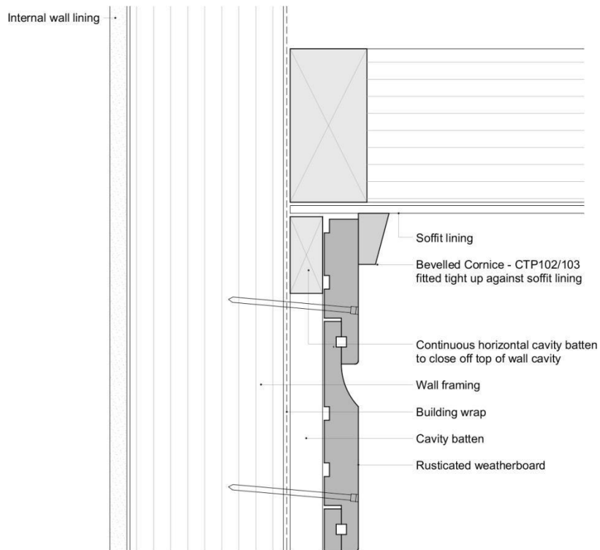
Rusticated – Top Of Wall – Flat Soffit
