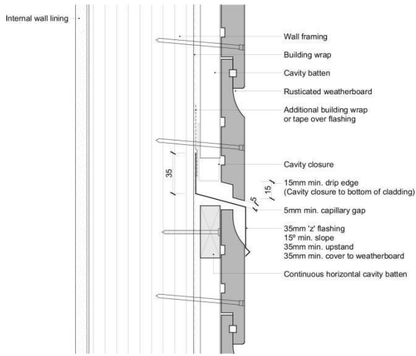
Rusticated – Inter-Storey Cavity Junction
