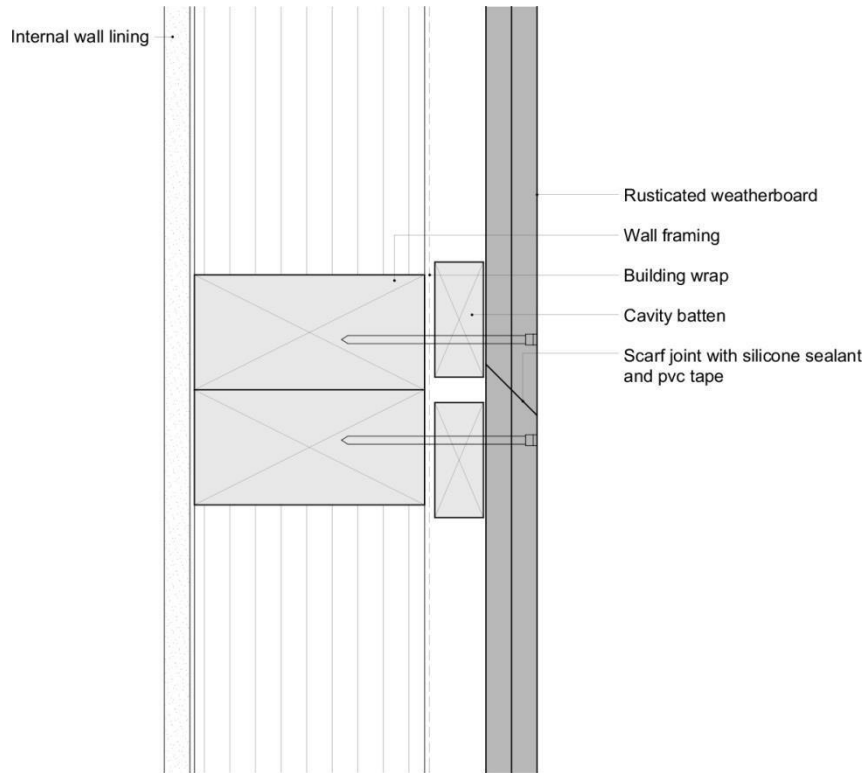
Rusticated – Weatherboard Join
