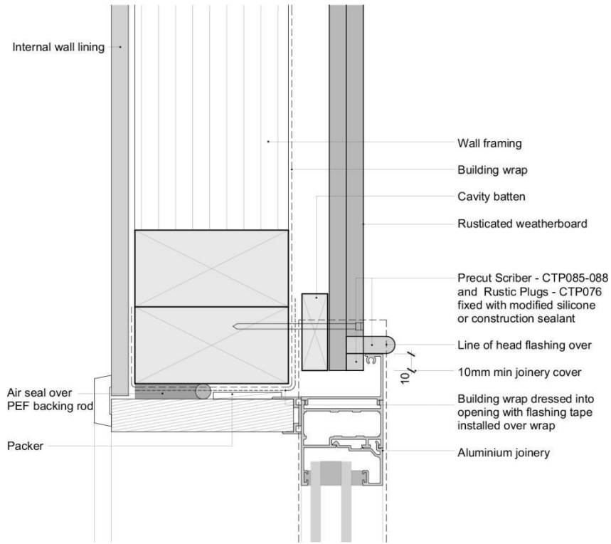
Rusticated – Window Jamb
