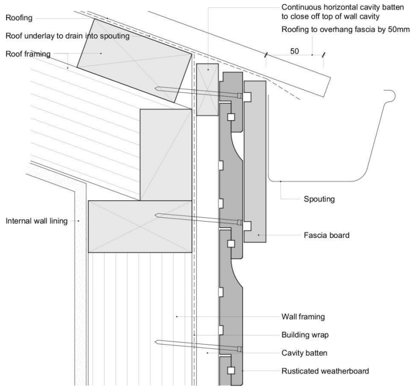
Rusticated – Top Of Wall – No Soffit
