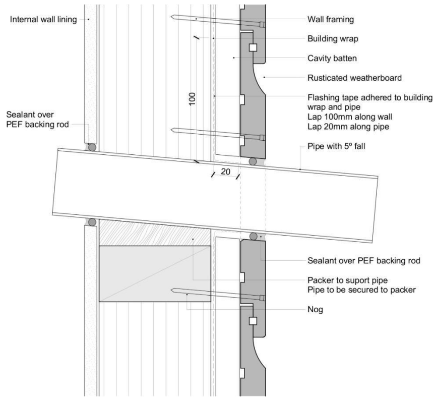
Rusticated – Pipe Penetration
