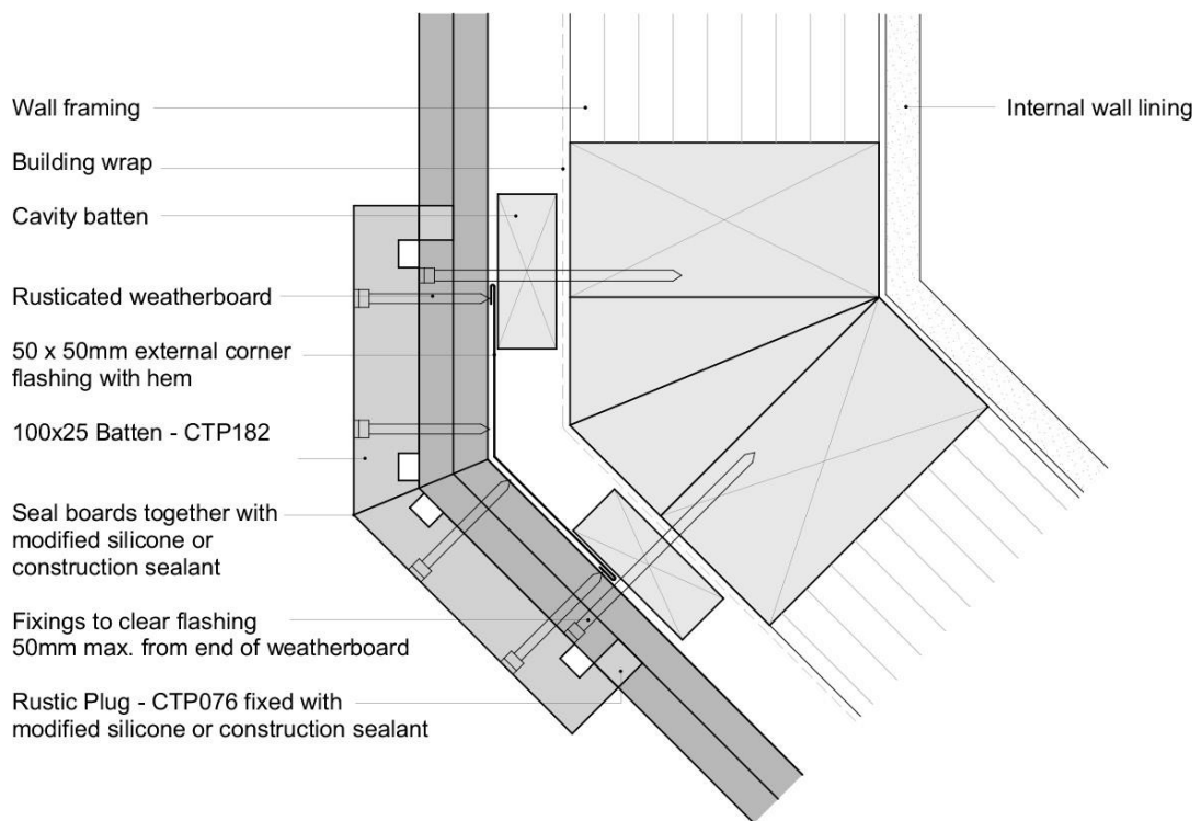
Rusticated – External 135° Corner – Boxed
