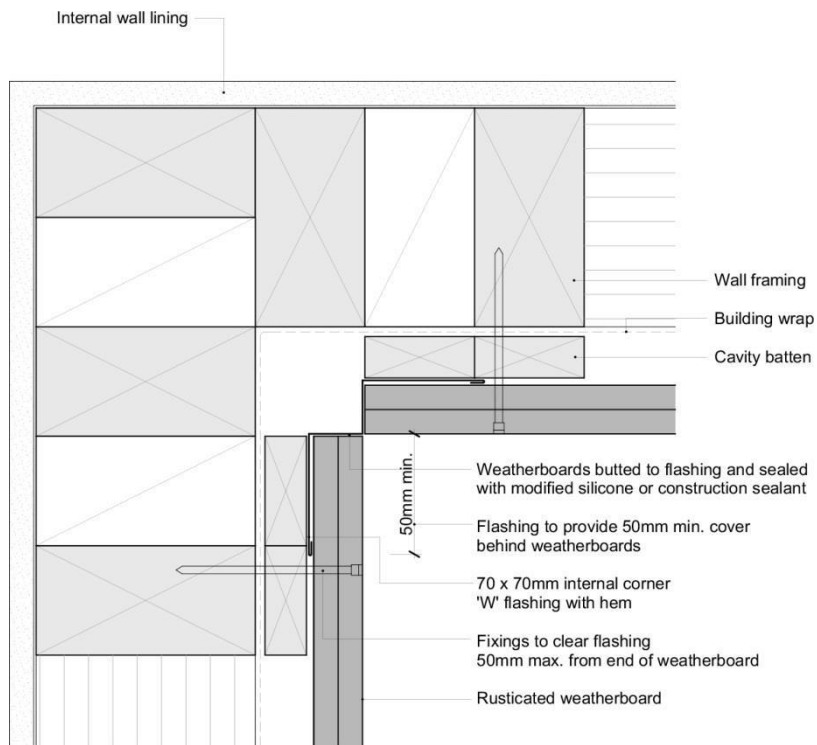
Rusticated – Internal 90° Corner – Flashing
