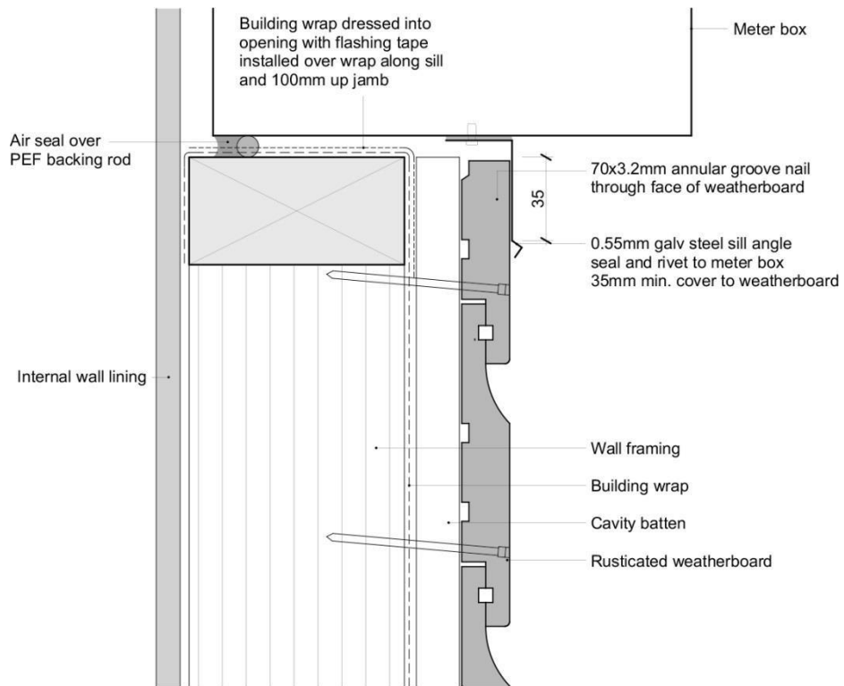
Rusticated – Meter Box Sill
