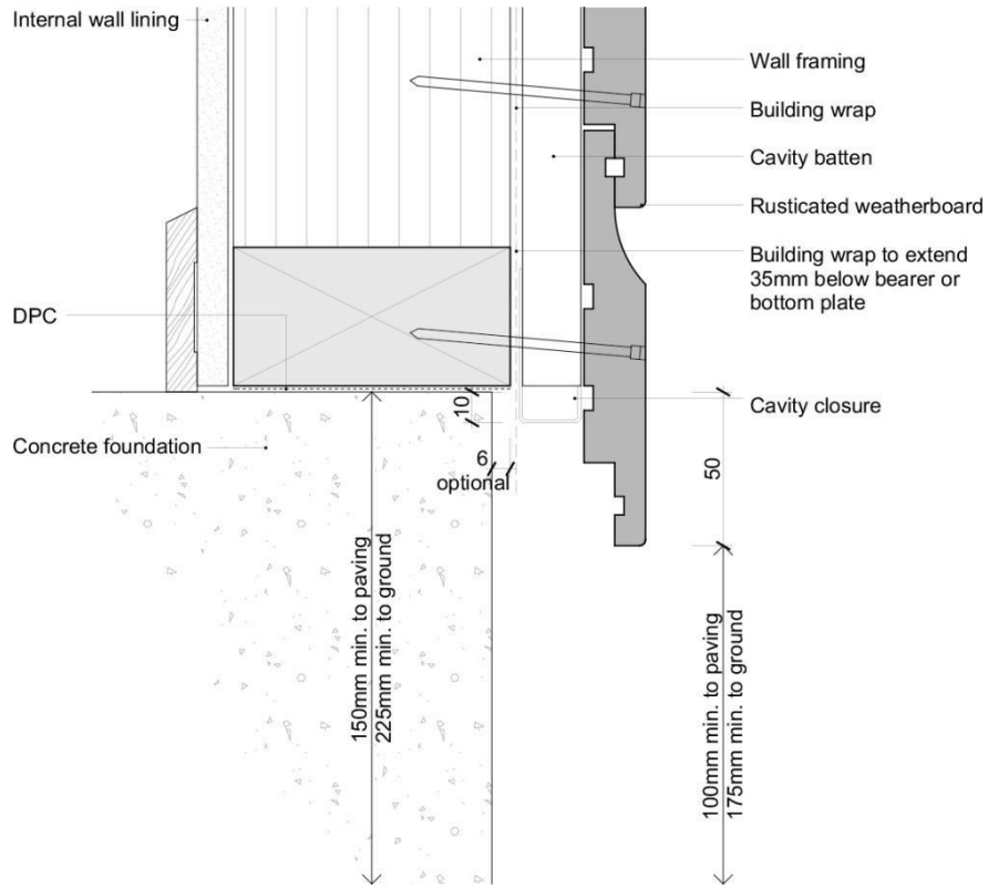
Rusticated – Base Of Wall – Concrete Floor
