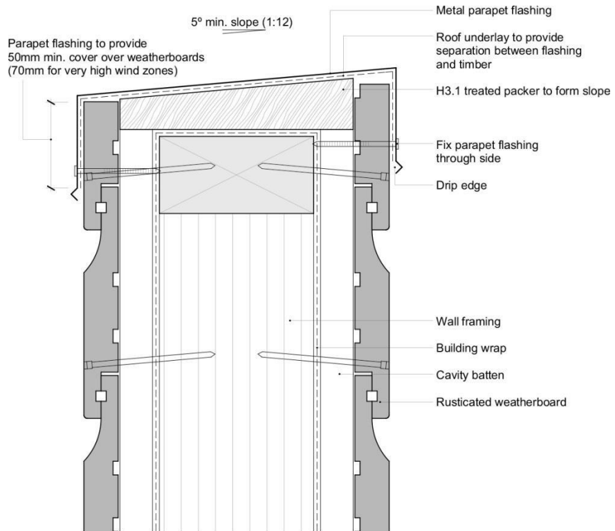
Rusticated – Parapet Balustrade Cap Flashing
