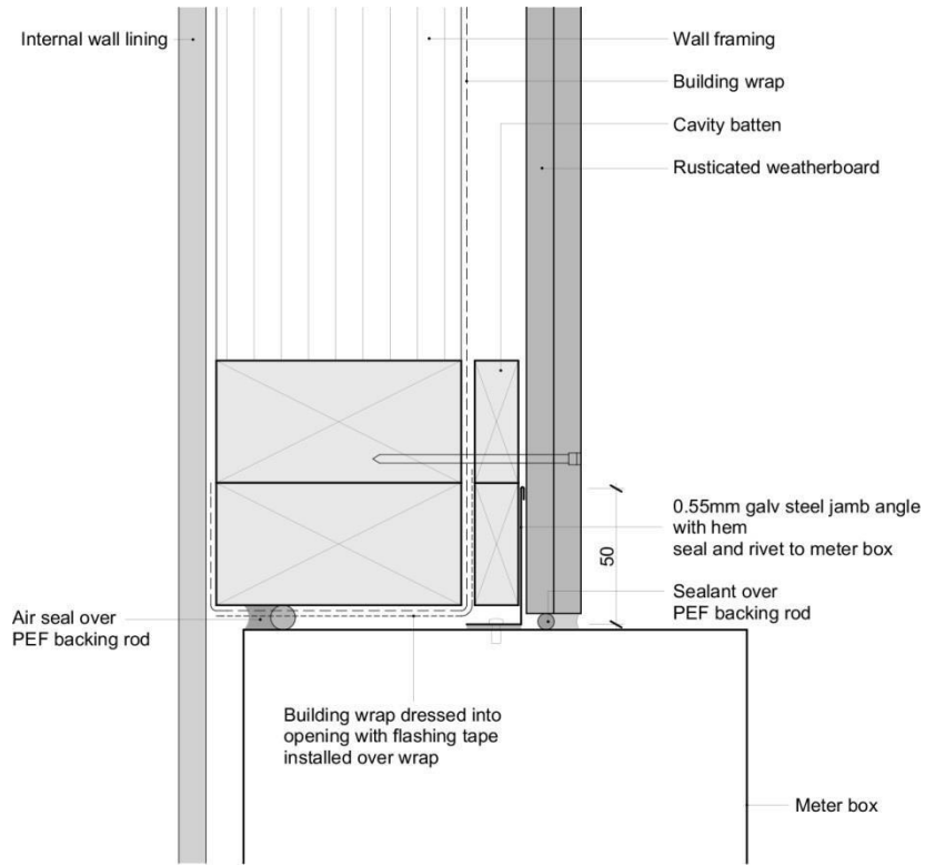
Rusticated – Meter Box Jamb
