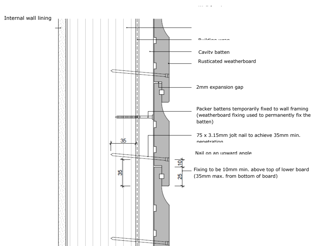
Rusticated Fixing
