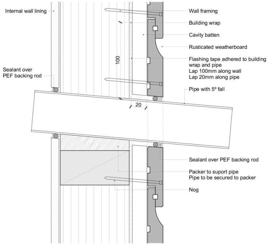
Rusticated – Pipe Penetration
