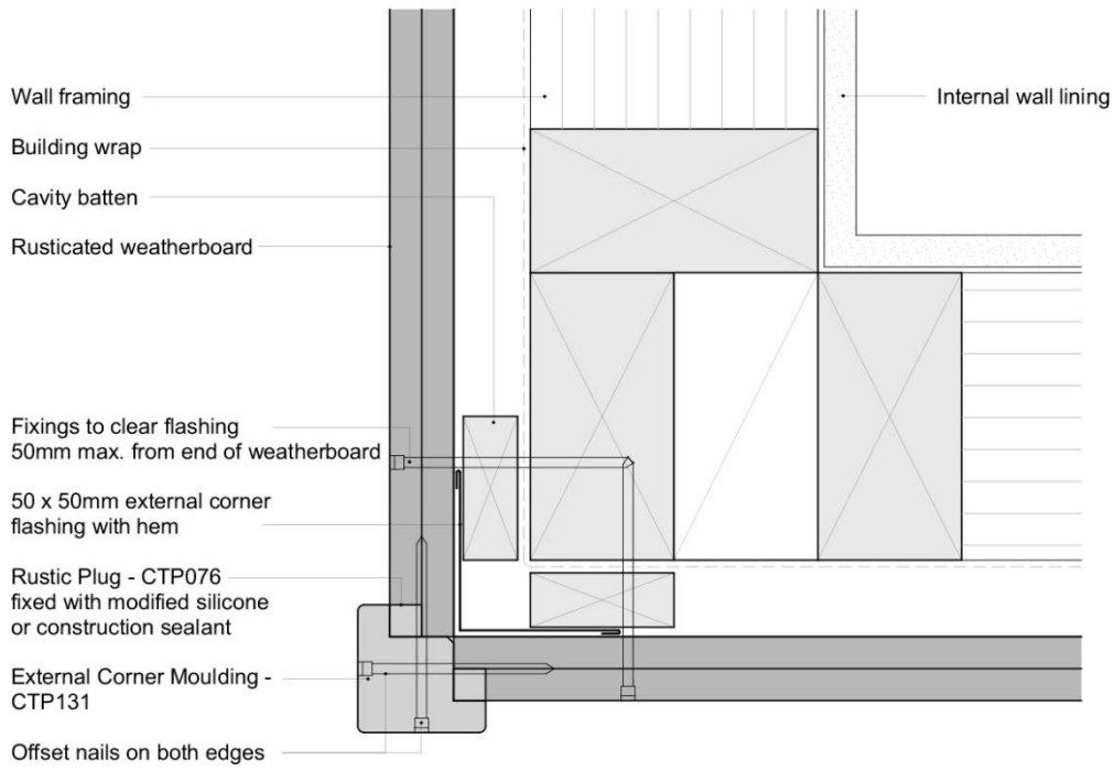
Rusticated – External 90° Corner – Moulding
